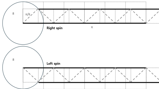
Fig.9. A planar diagram made of 8 isosceles triangles (16 right triangles). The upper part represents right spin, and the lower part represents opposite spin. If the upper part is an electron, the lower part can be viewed as a positron.
