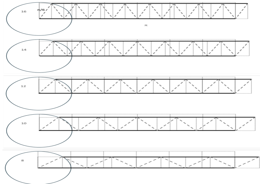
Fig.4. Planar view of a three-dimensional shape that can be folded from a strip with an area of \pi^2/6 .
