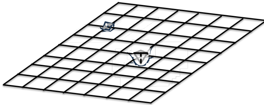
Fig.16. A universe with a 2-dimensional photon field.
