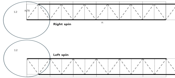
Fig.5. Floor plan created by 12 equilateral triangles. The top has a right spin and the bottom has an opposite spin.
