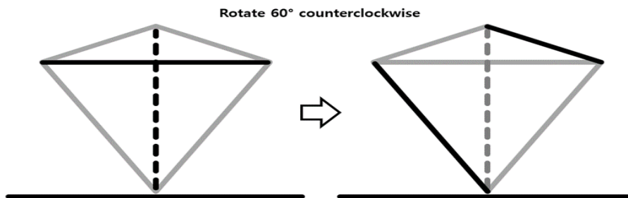
Fig.7. View of the tetrahedral model existing in the reverse direction
