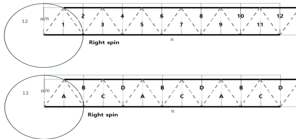
Fig.6. The number of overlaps (numbers) for each face (alphabet) in the proton model.
