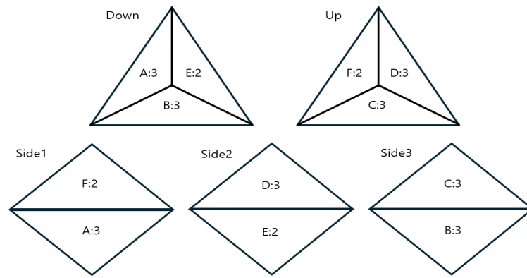
Fig.11. Top/bottom/side views of the electron, showing the order of faces (alphabet): number of overlaps (numbers).
