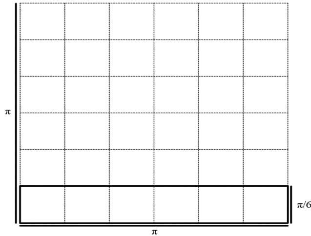
Fig.1. A strip shape covering 1/6 of a square with one side of length \pi .
