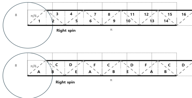
Fig.10. The number of overlaps (numbers) for each face (alphabet) in the electron model.
