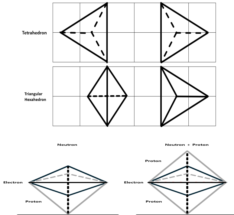
Fig.14. A tetrahedron and triangular hexahedron made from a strip with a height of \pi/6 fit together perfectly. (Top) This shape becomes the shape of a neutron when a proton and an electron combine (Bottom left), and when a proton is overlaid, the electron cannot escape and becomes stabilized. (Bottom right).
